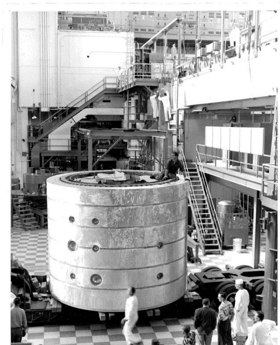
Moving Vessel No. 2 into reactor hall. 1966 September.
